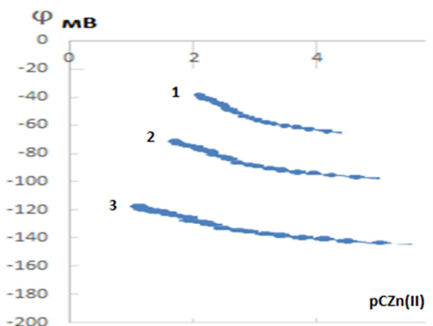
Figure 1. \varphi - pC_{Zn^{2+}} dependence. System: Zn(II) - ACC - Na(H)SO 4 - H 2 O 308K; I=0.1 mol/l; pH: 1) 5,0 2) 6,0 3) 7,0 C ACC = 1 \cdot 10^{-2} mol/l.
