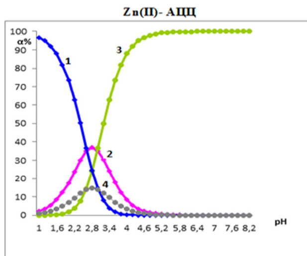
Figure 5. The content of the Zn (II) ions and its complex forms in the system: Zn (II) - Zn (0) -ACC- H_2O , 308 K; J=0.1 mol / l.
