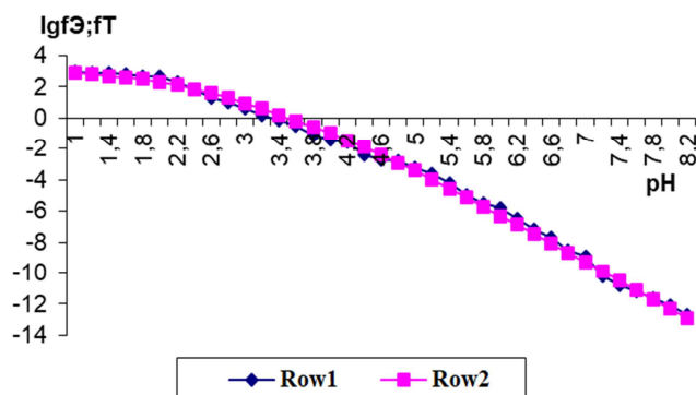
Figure 4. The dependence of the experimental ( Igf_{\tau}^0 ) and theoretical ( Igf_{\tau}^0 ) oxidation functions on pH in the system: Zn (II) - Zn (0) - ACC-H 2 O, 308 K, J=0,1 mol/l, C_{Zn(II)}=1 \cdot 10^{-3} , C_{ACC}=1 \cdot 10^{-2} mol/l.
