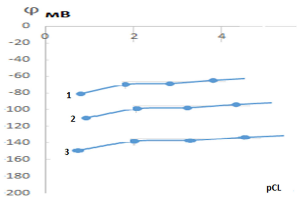
Figure 2. \varphi - pC_{ACC} dependence. System: Zn (II) - ACC - Na(H)SO 4 - H 2 O 308K; I=0.1 mol/l; pH: 1) 5,0 2) 6,0 3) 7,0 C Zn 2+ = 1 \cdot 10^{-3} mol/l.
